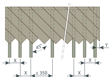
fig.2: Installation 45°
